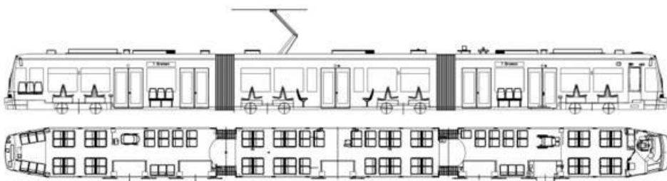
Seat configuration FLEXITY CLASSIC Bremen
