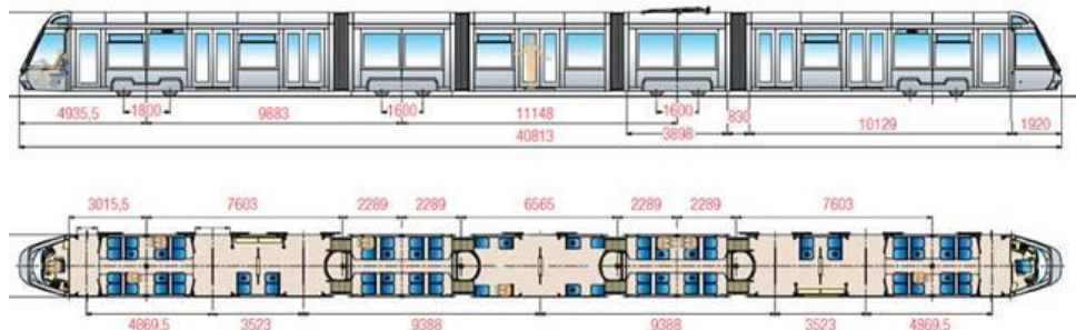
Seat configuration CITADIS Dublin
